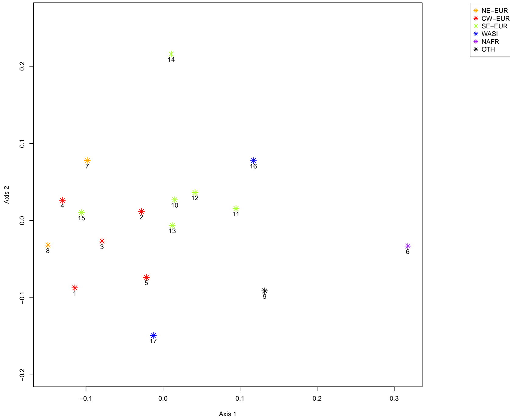
2nd-field HLA-DPB1 data (stress=0.1291)
