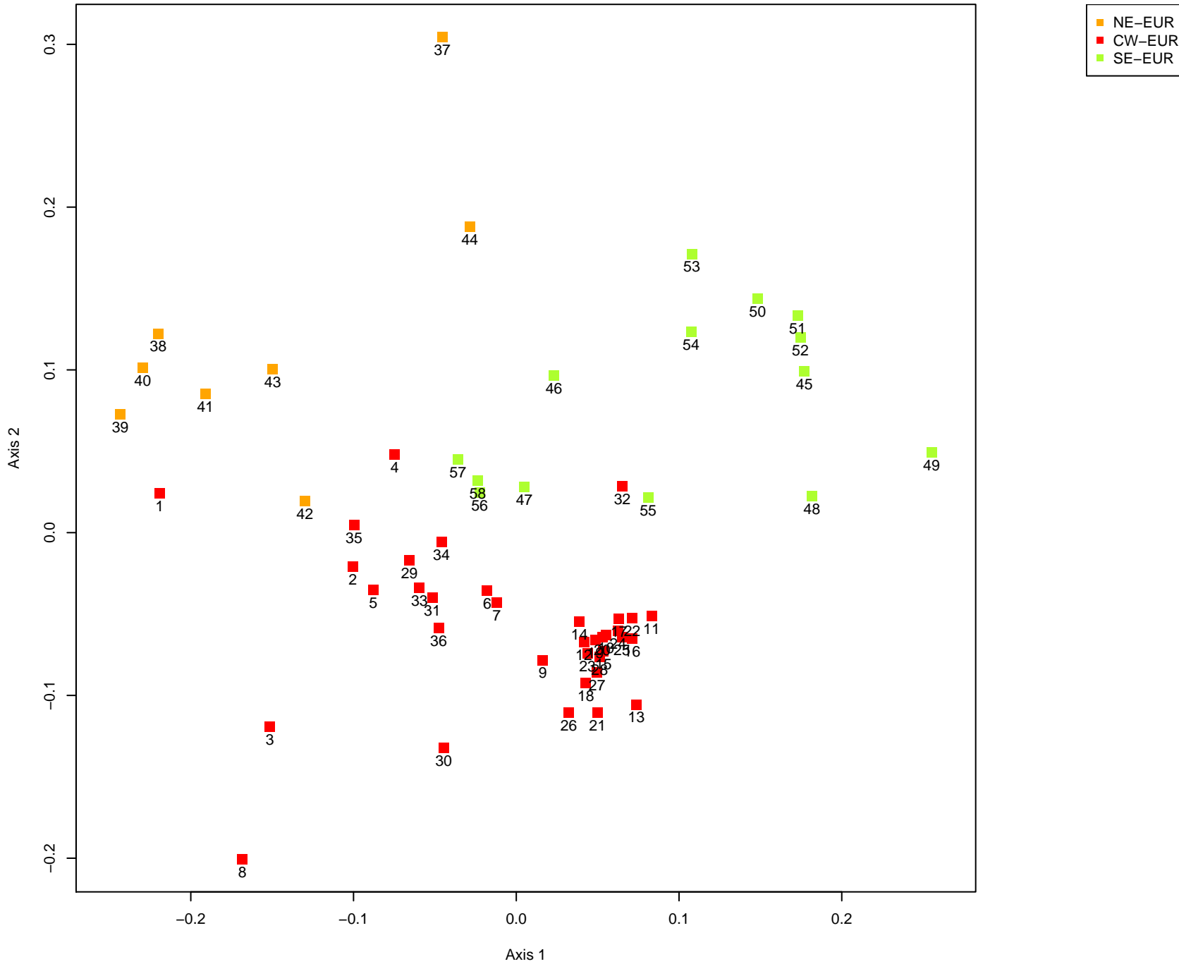
1st-field HLA-B data (stress=0.1187)
