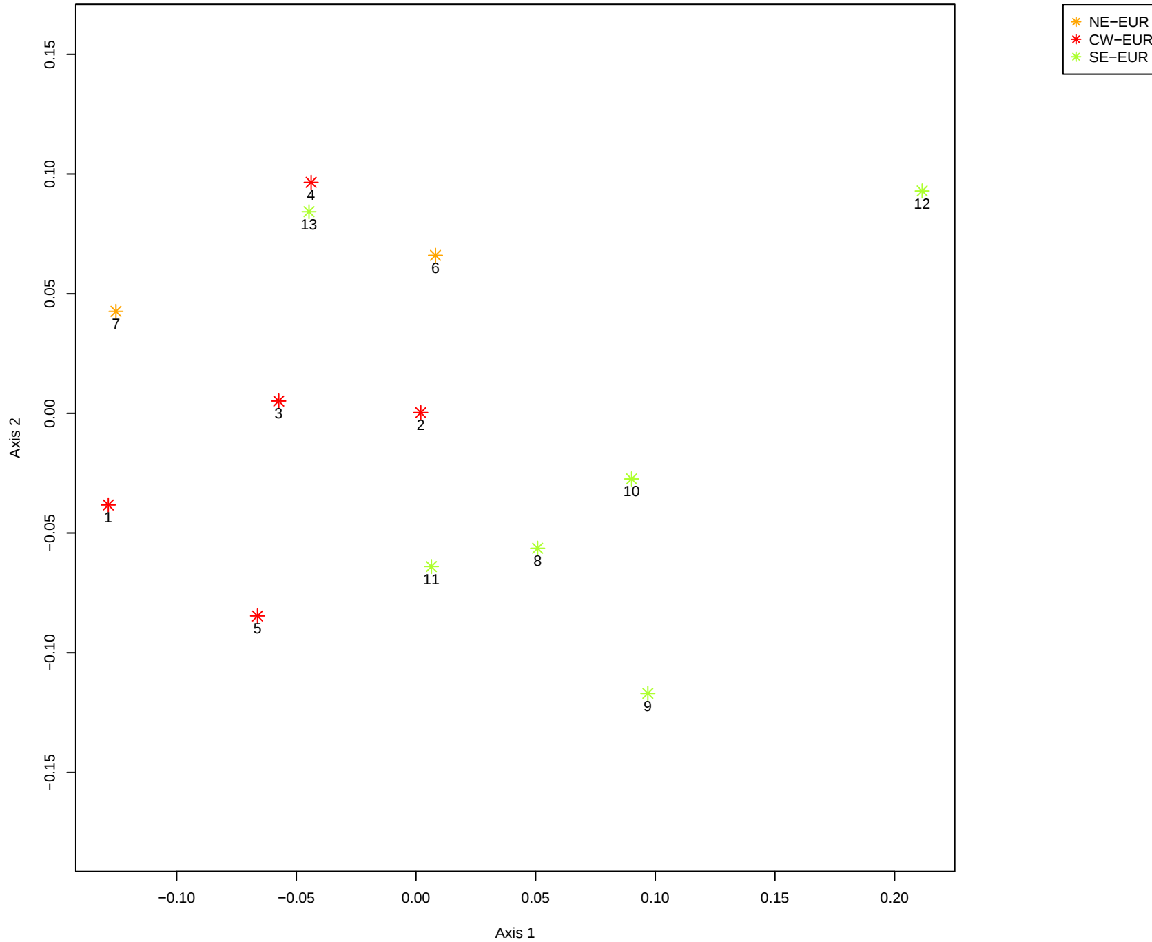
2nd-field HLA-DPB1 data (stress=0.1119)
